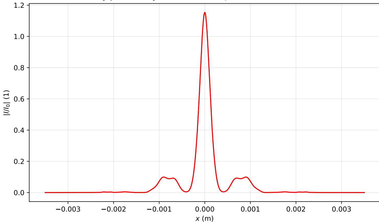
Intensity profile I(x, y = 0, z = 1.672)/I_0 , P_{in}=8.5P_{cr} , artificial time
